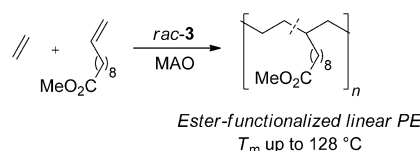
Scheme 3. Copolymerization of ethylene and methyl 10-undecenoate using rac-3 .
